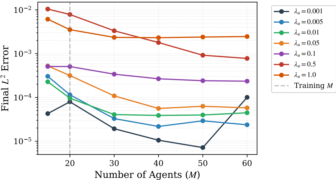
Zero-Shot Scalability: Tracking MSE
